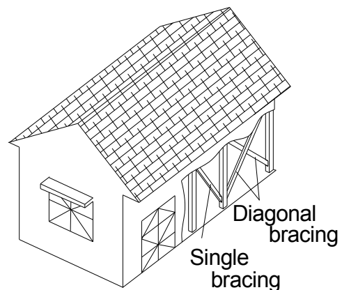
Reinforcement by wooden bracing
